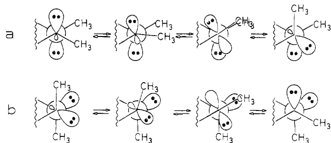
Figure 2. Diagram contrasting lone-pair–lone-pair interactions for the high- and low-barrier nitrogen inversion of hexahydro-pyridazines. (a) The ee \rightleftharpoons ae' conversion (high barrier). (b) The aa \rightleftharpoons ea conversion (low barrier).
